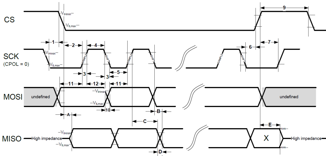
Figure 3: NEO-M9N-00B SPI specification mode 1: CPHA=0 SCK = 5.33 MHz
