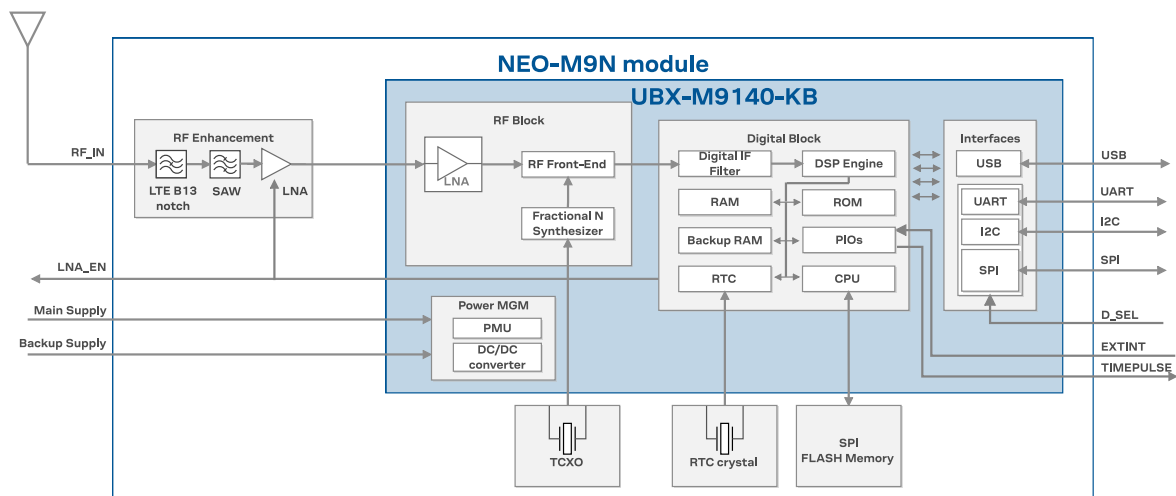
Figure 1: NEO-M9N-00B block diagram
