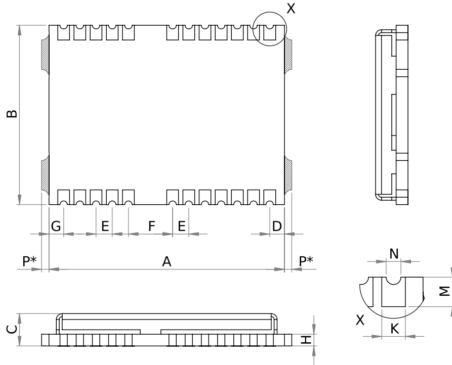
Figure 5: NEO-M9N-00B mechanical drawing
