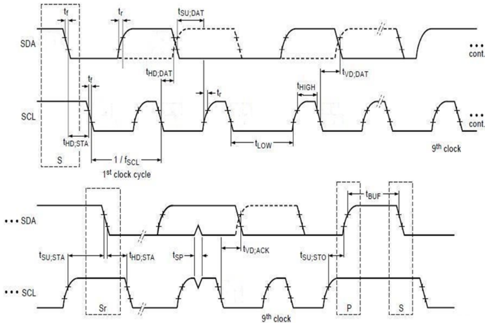
Figure 4: NEO-M9N-00B I2C slave specification
